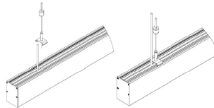
Suspension Kit Mounting Illustration
