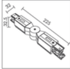
CTA006 - JOINING CONNECTOR MINI (CENTRAL FEED)
