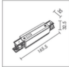
CTA003 - JOINING CONNECTOR (CENTRAL FEED)
