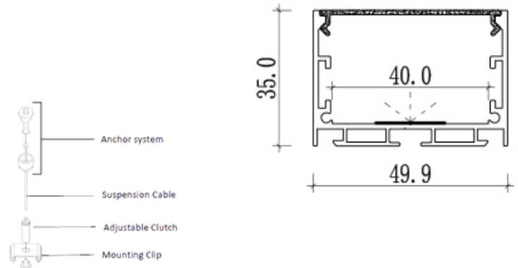
Suspension Kit Mounting Illustration
