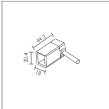
QUICK CONNECTOR WITH WIRE IN THE MIDDLE
