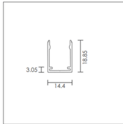
FLAT MOUNTING ALUMINIUM GROOVE 1000MM
