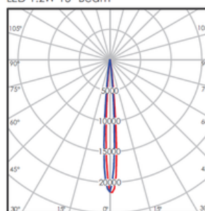
LED 1.2W 15° Beam
