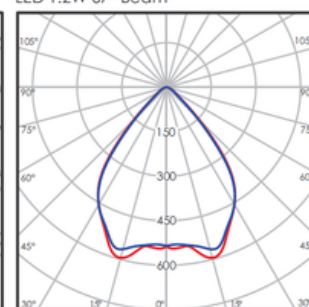
LED 1.2W 67° Beam
