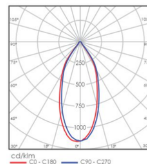
LED 20W 45° Beam
